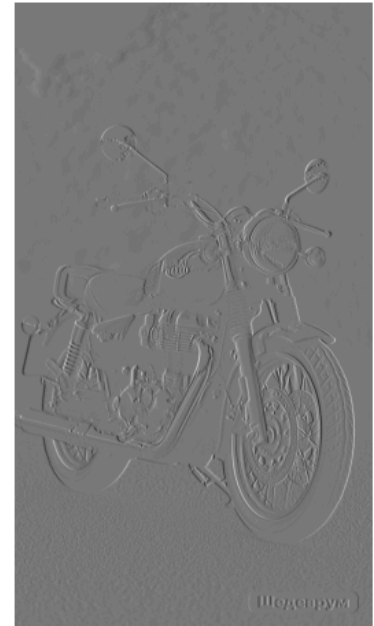
Prewitt Combined
