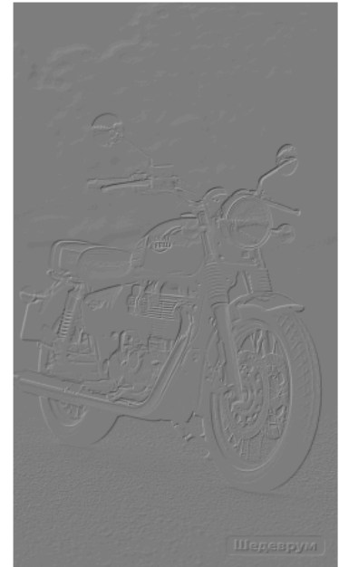
Robert Combined
