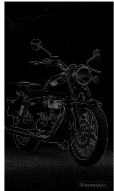
Robert Combined
